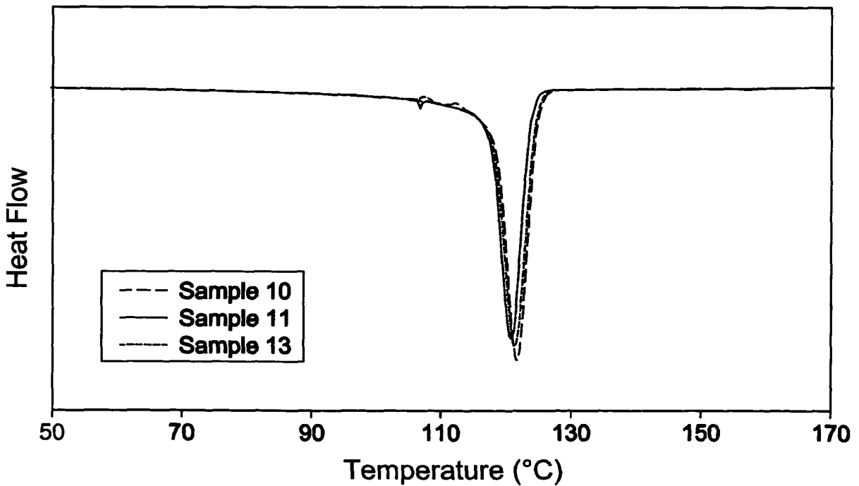
Fig. 8 DSC Crystallization of Plasticized Propylene Random Copolymers
